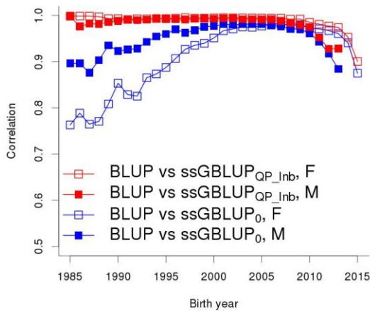
Figure 3. For ICF2, annual EBV and GEBV correlations for both females (F) and males (M).
