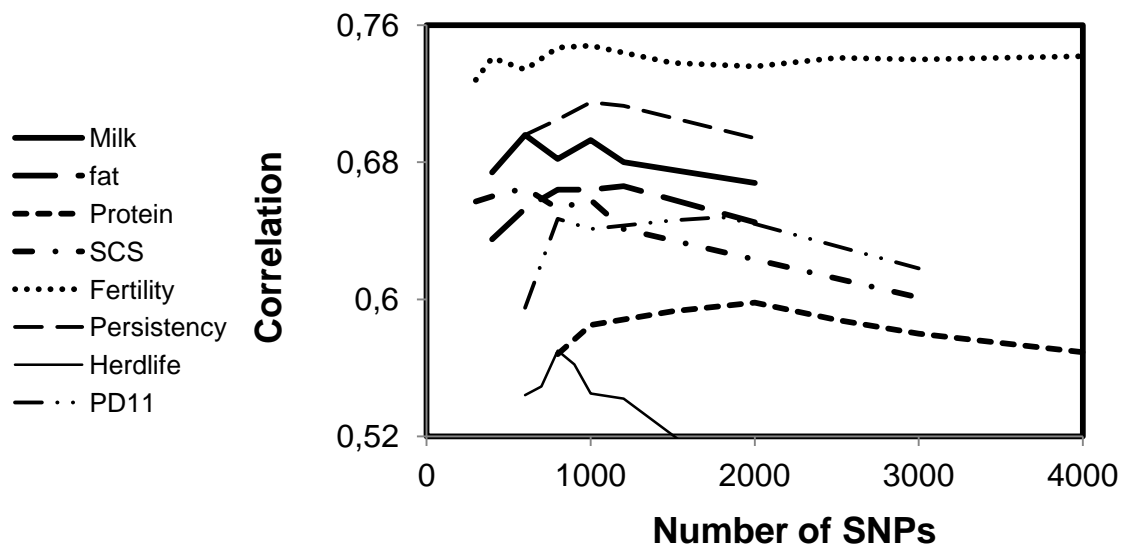
Figure 2. Correlations between Method 1 GEBV and current EBV as a function of the numbers of SNPs included in the analysis.
